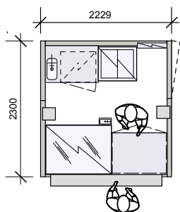
TOPBOX 23 ICE CREAM
